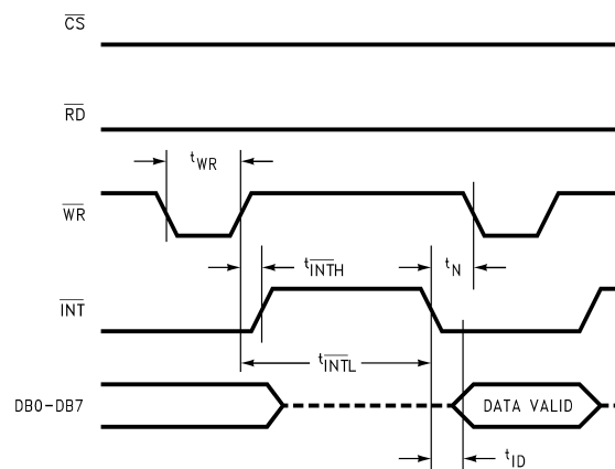
Figure 4. \overline{\text{WR}}\text{-}\overline{\text{RD}} Mode Reduced Interface System Connection with \overline{\text{CS}} = \overline{\text{RD}} = 0 (Mode Pin is High)
